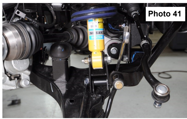
Install Strut Assembly On Lower Control Arm
