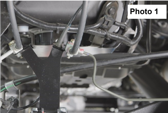
Install Rear Brake Line Bracket Off Rear Axle
