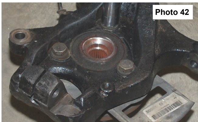
Remove Wheel Bearing Assembly from Stock Knuckle
