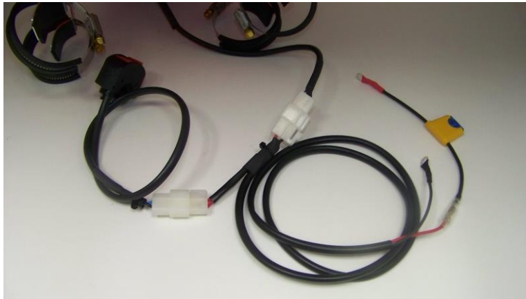
Baja Designs harness w/switch part# 61-1049
